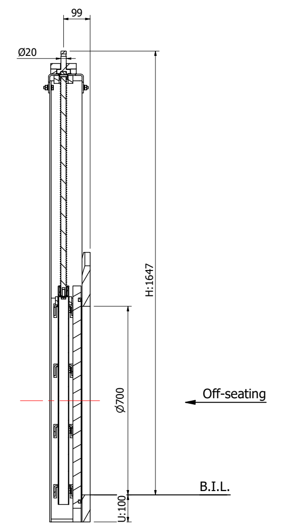
Section view A-A
