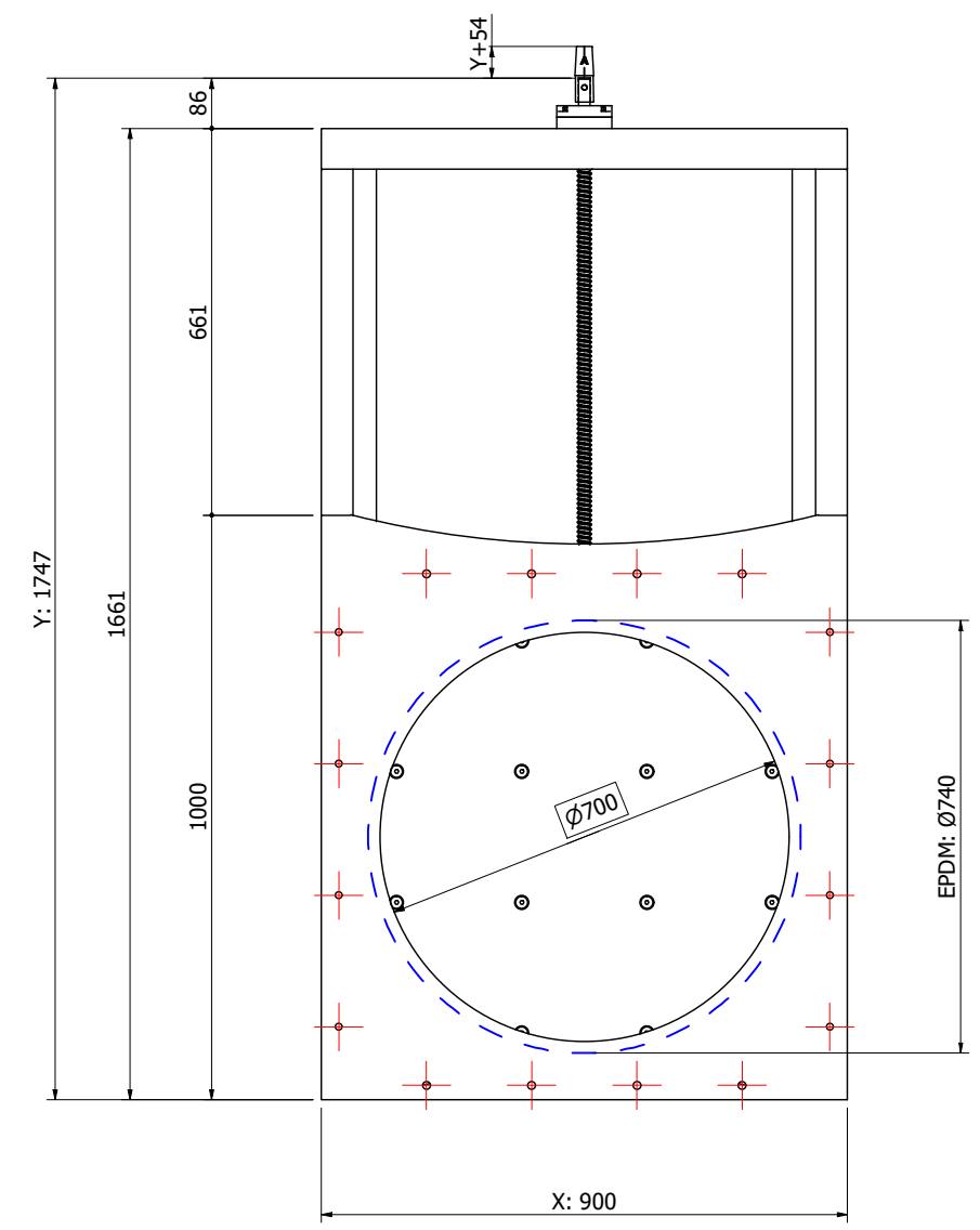
Back view
