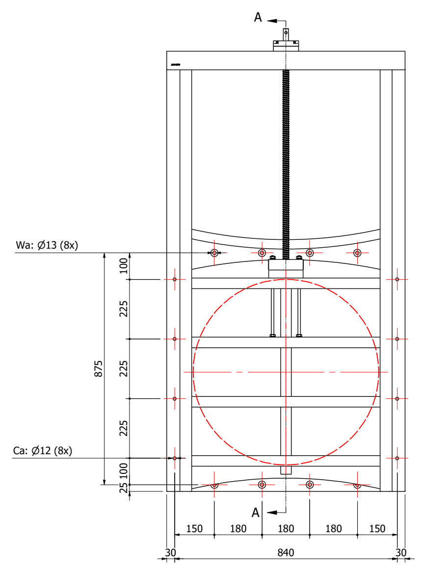
Front view
