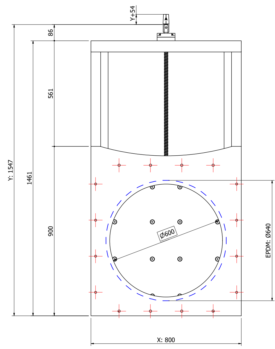
Back view
