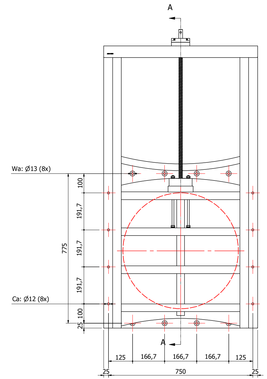
Front view
